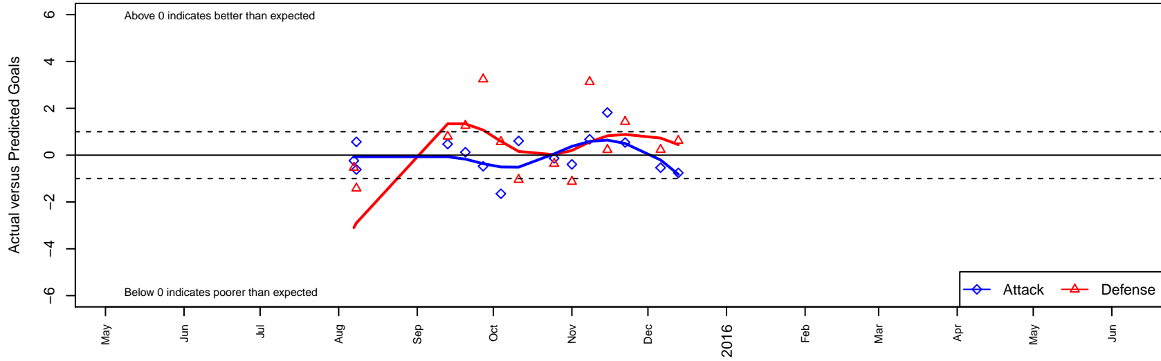
FWFC Sharks B00 Dots are actual minus expected GF (blue circles) and GA (red triangles). Blue line is smoothed change in attack strength. Red is smoothed change in defense strength.
